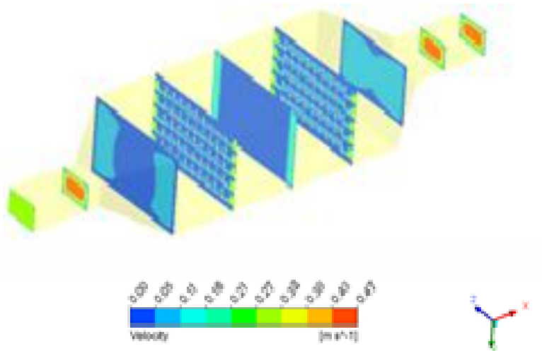
Figure 14. Velocity contour.
