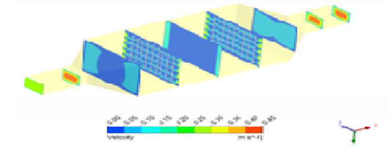
Figure 8. Velocity contour.
