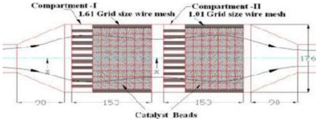
Figure 1. Catalytic converter Showing Two Compartments
