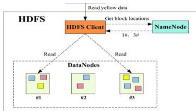
Figure 1. HDFS Architecture.
