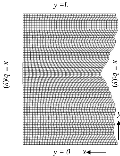
Figure 1. Boundary fitted grids in physical domain.
