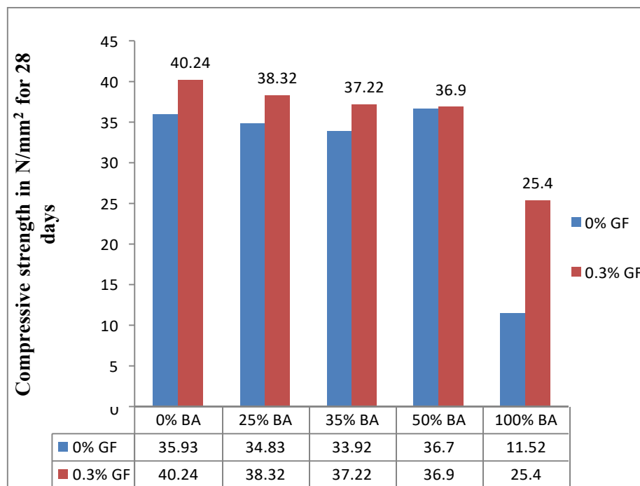
Fig 8.2 Compressive Strength Results in N/mm 2 for 28 days
