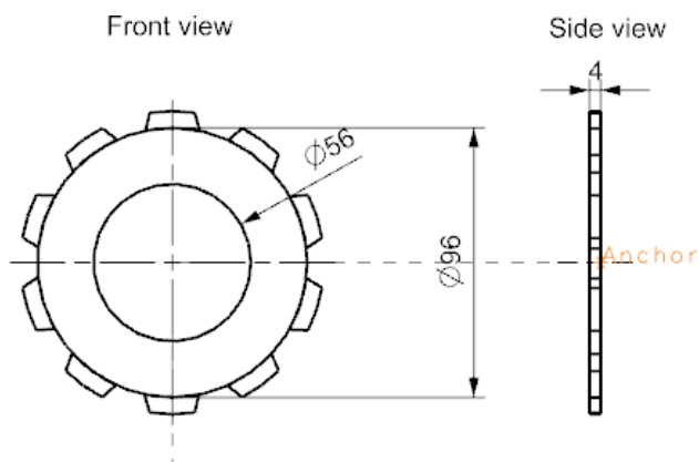
Fig.1. Orthographic view of clutch plate
