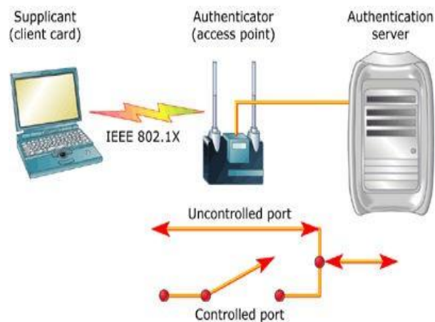
FIG.3 802.11i SECURITY
