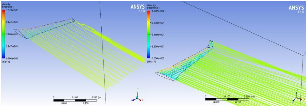
Fig.13: Velocity streamline 3° AOA
