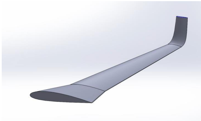
Fig.5: Wing with Winglet Model
