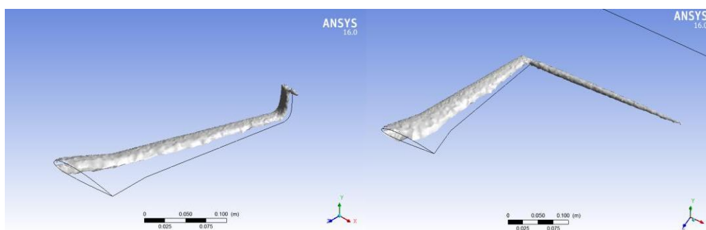
Fig.10: Core Vortex region at 3° AOA with and without winglets
