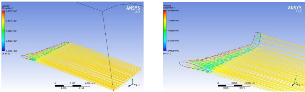
Fig.12: Velocity streamline 0° AOA
