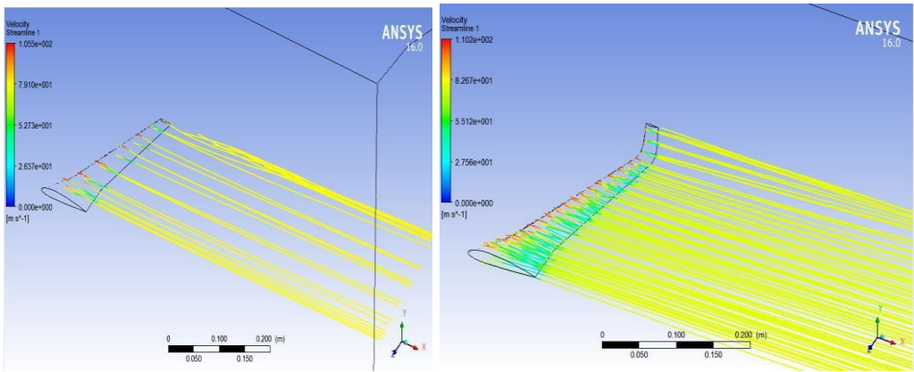
Fig.13: Velocity streamline 3° AOA
