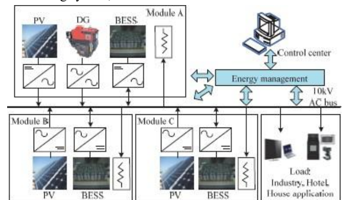
Fig : 1proposed hybrid micro-grid structure
