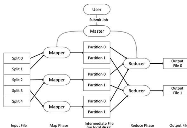
Fig. 1 Architecture of MapReduce Operation
