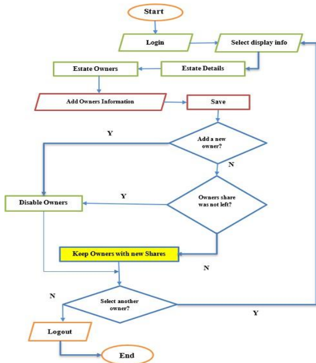
Fig. 4. Data flow diagram of EsOM
