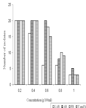
FIGURE8. Effect of different concentrations of ZnSO 4 on growth of isolates from spontaneously fermenting maize
