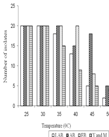
Figure 2: Effect of temperature on the growth of isolates from fermenting maize
